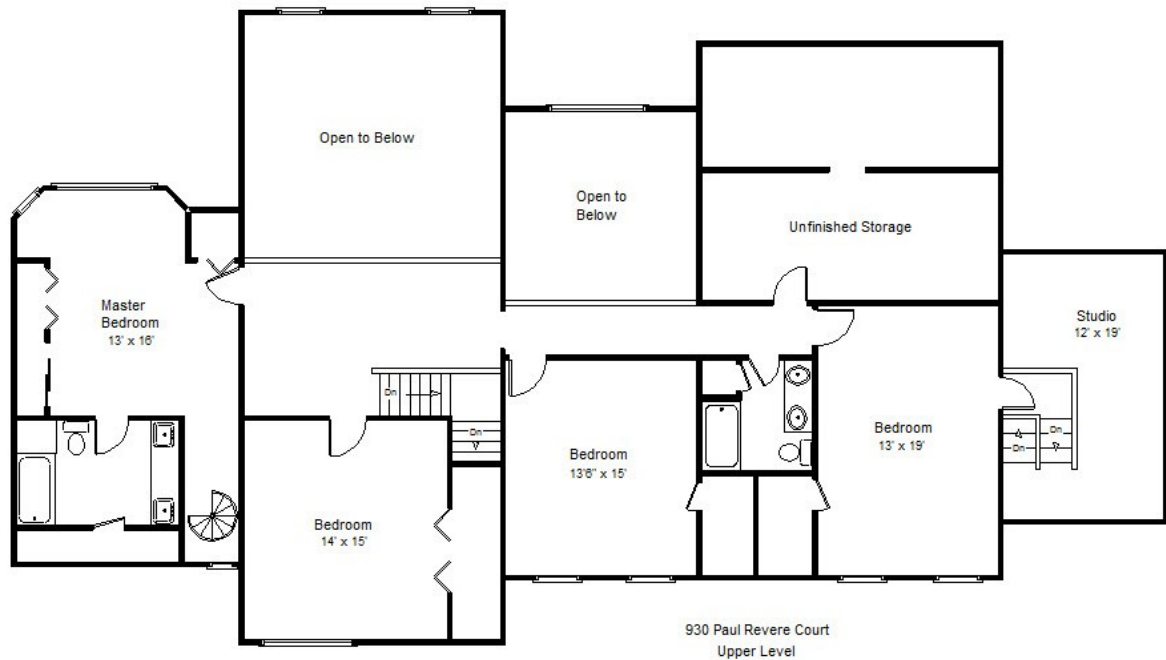
Top Floor
