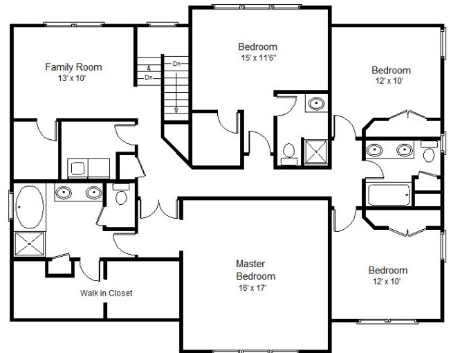
Top Floor
