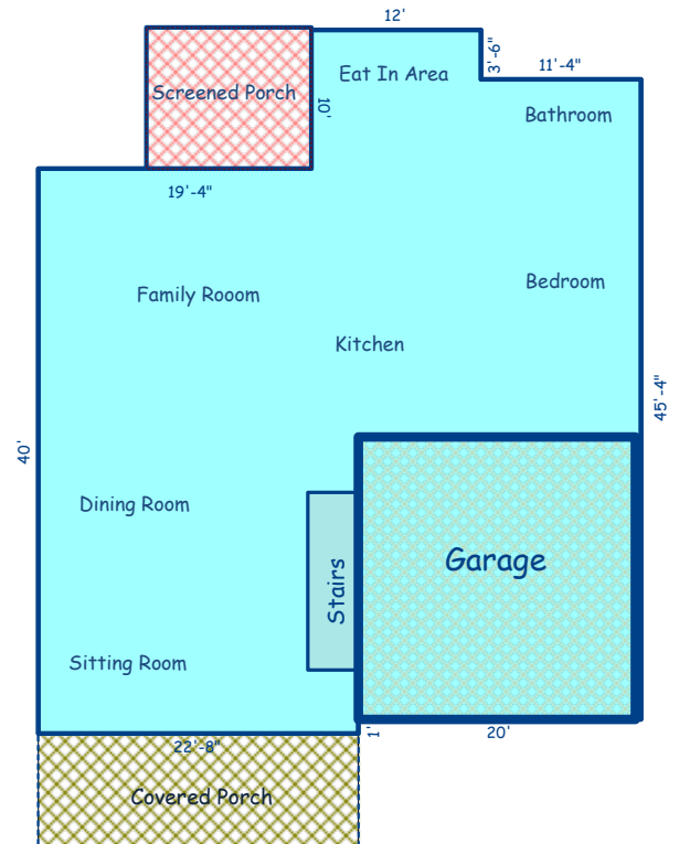
First Floor Aprx Gross living area: 1439.7 sf
