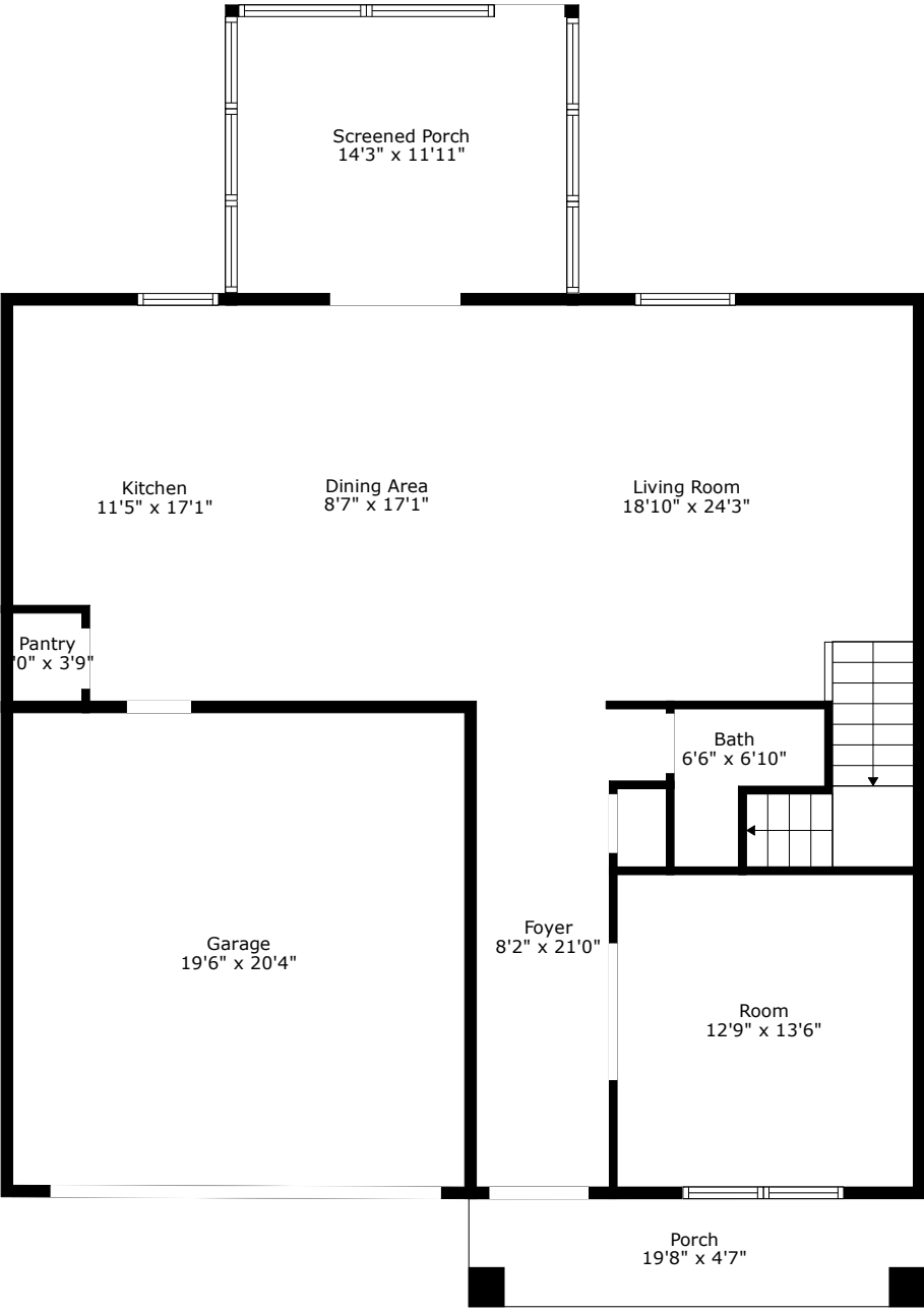
Floor 1
