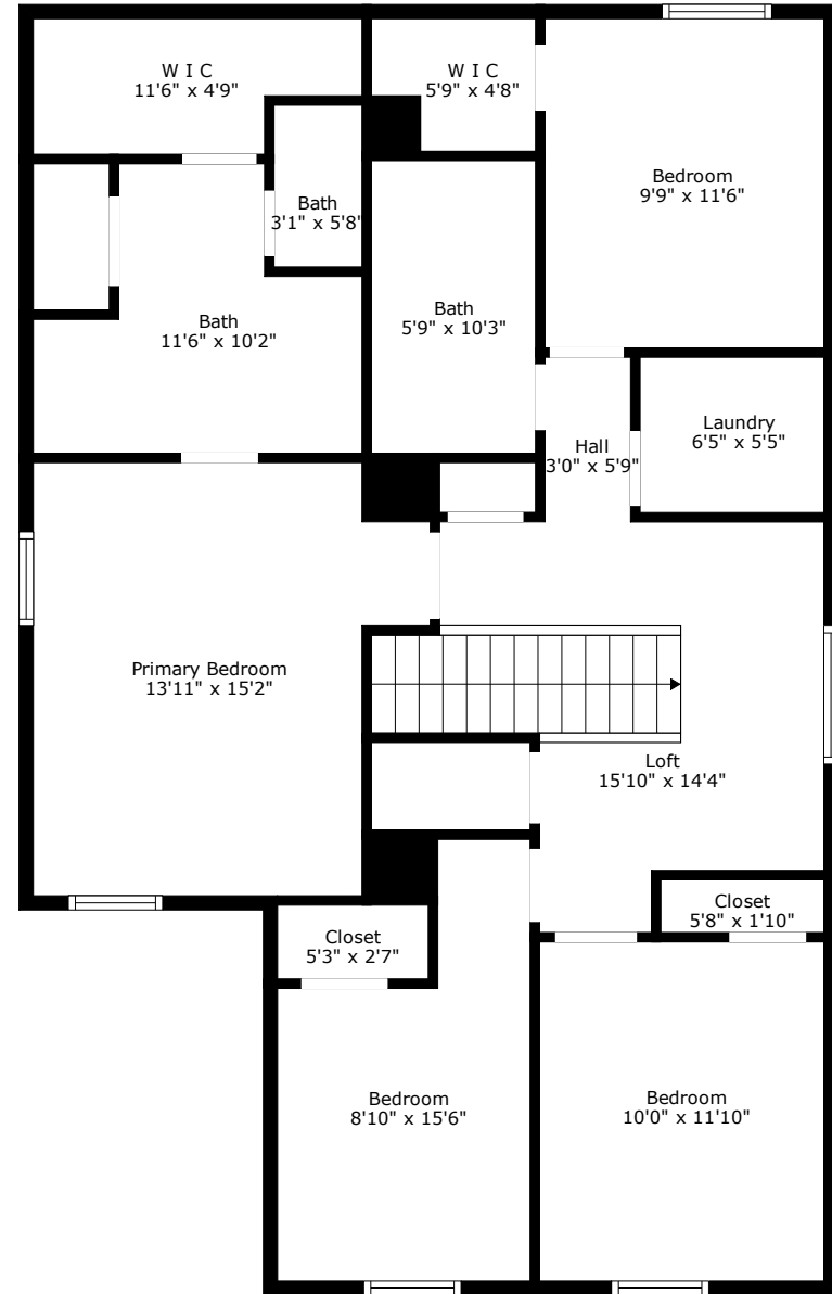
Floor 2
