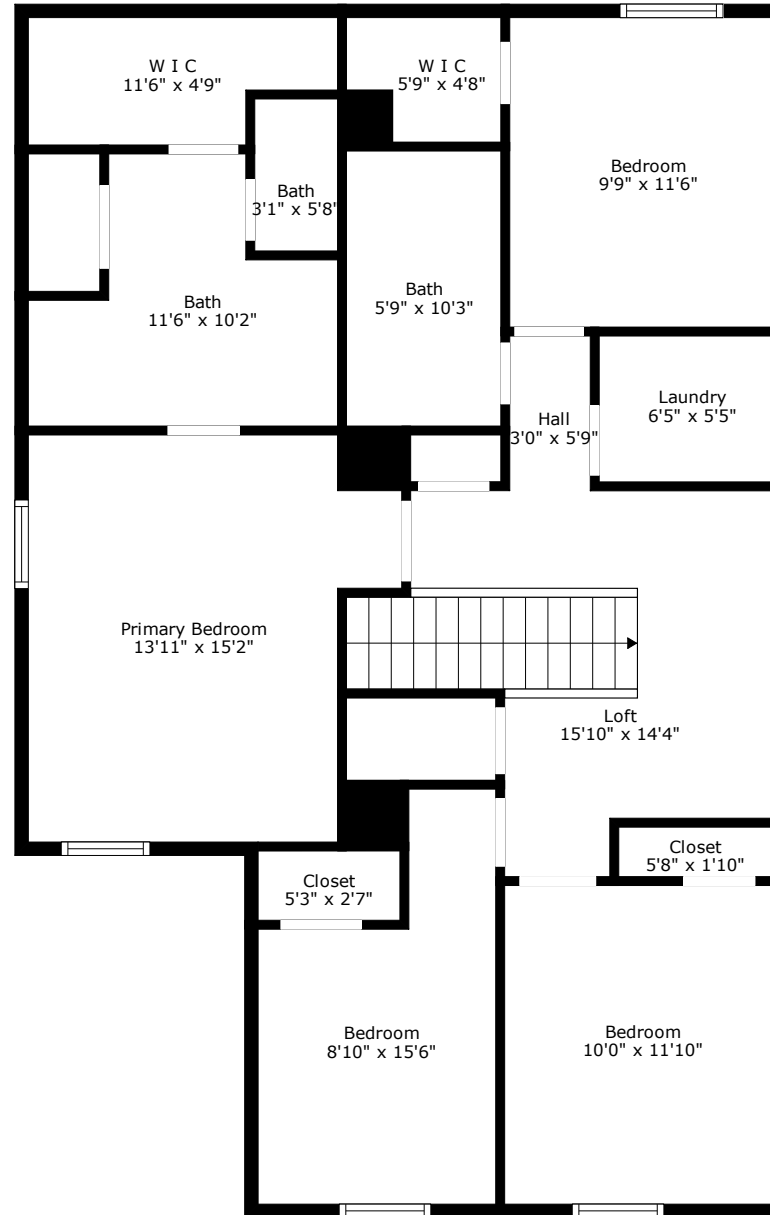
Floor 2
