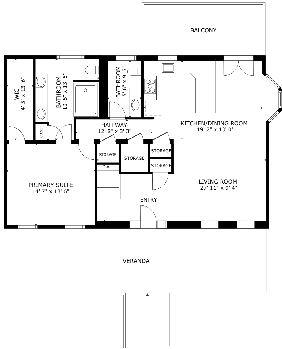
FLOOR 1
