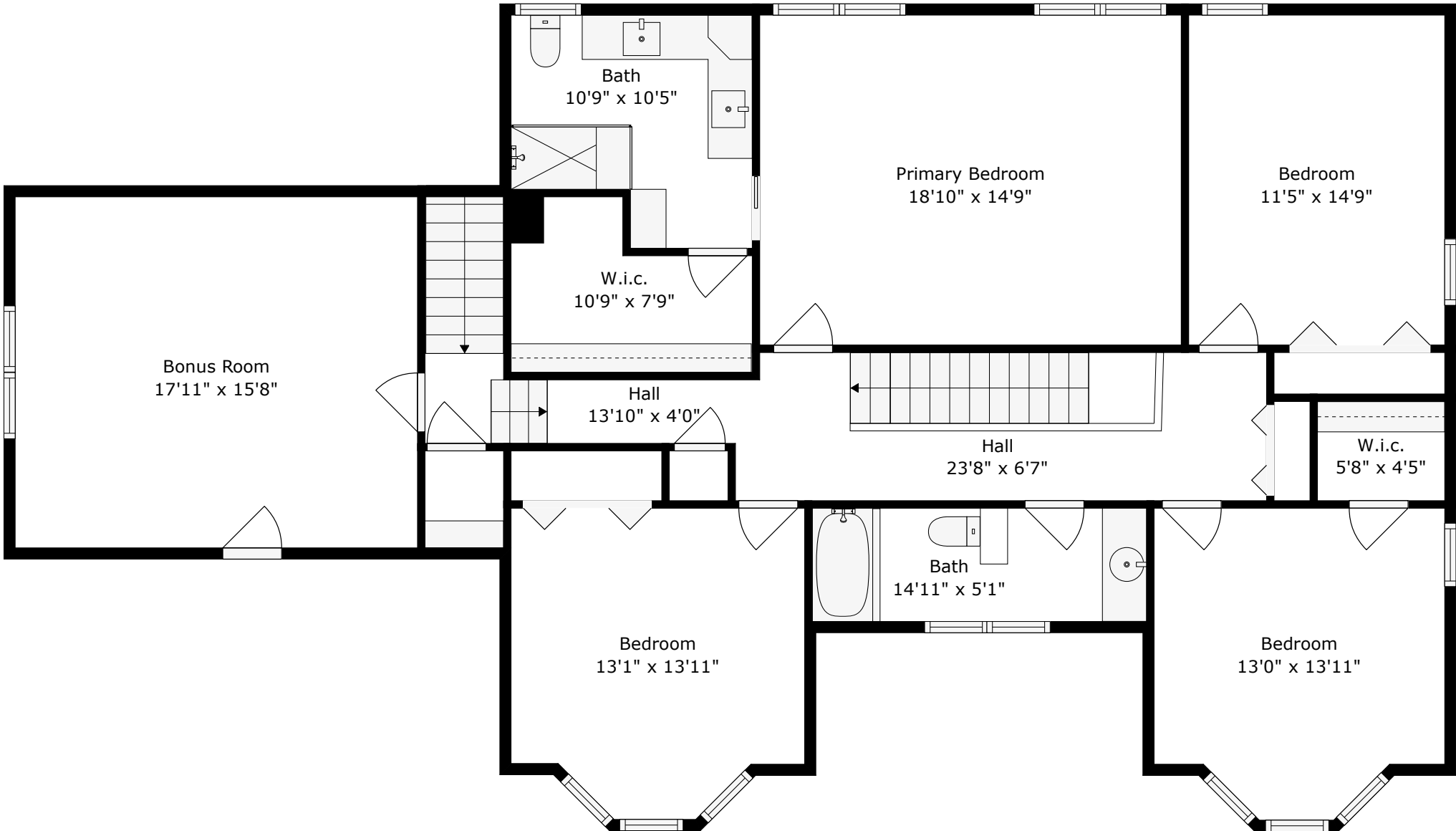
Floor 2
