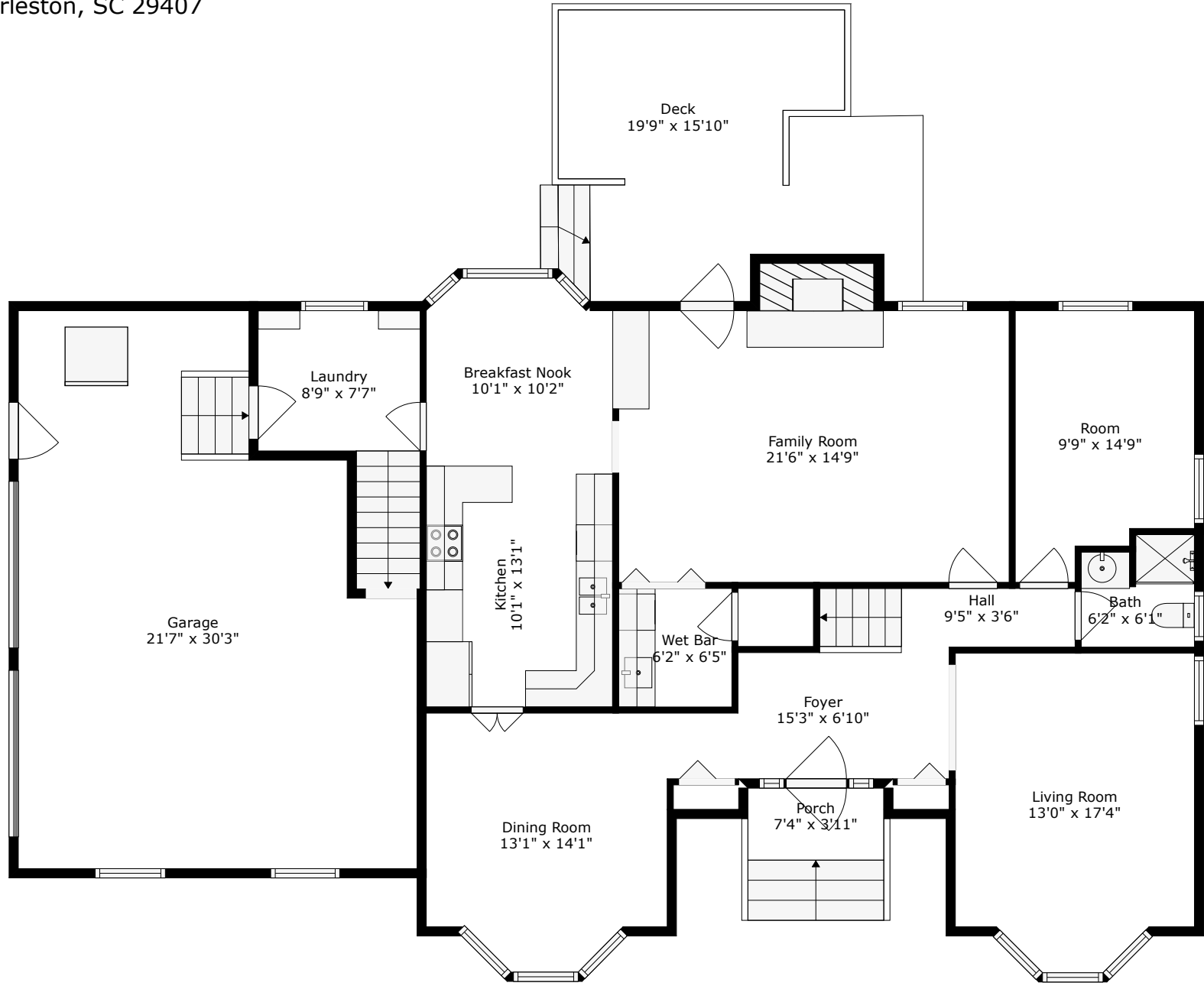
Floor 1
