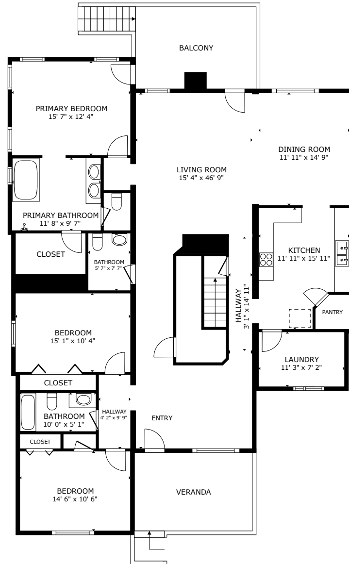
FLOOR 2
