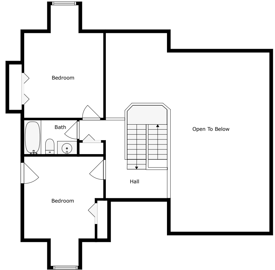
Floor 2
