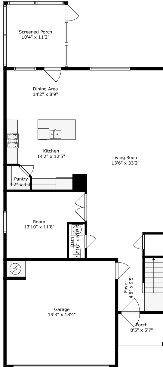
Floor 1
