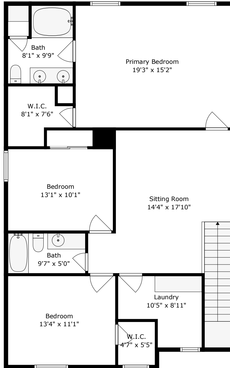
Floor 2
