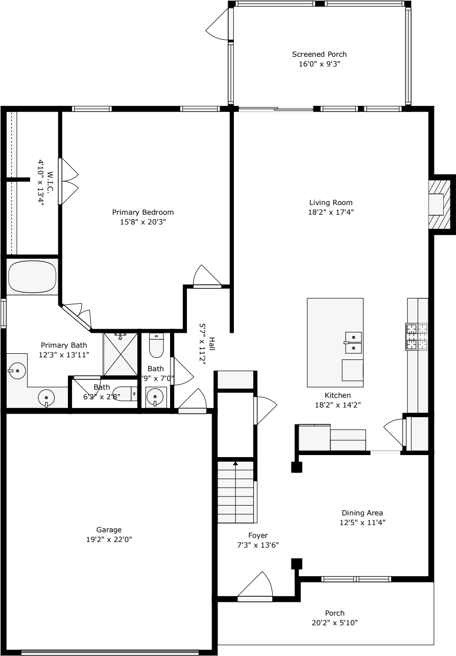
Floor 1
