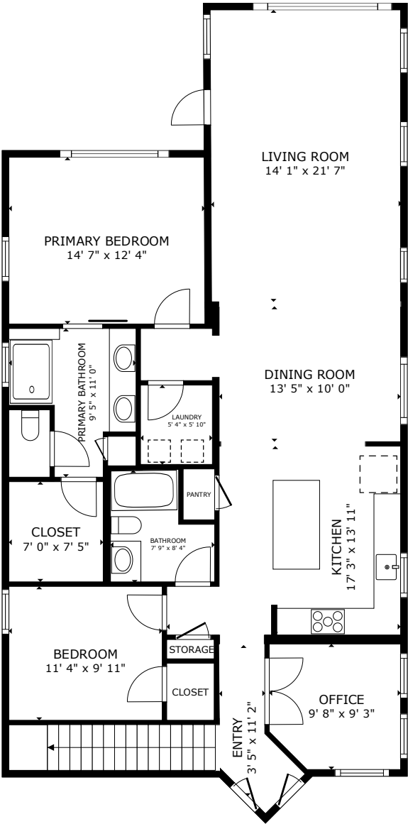
FLOOR 1
