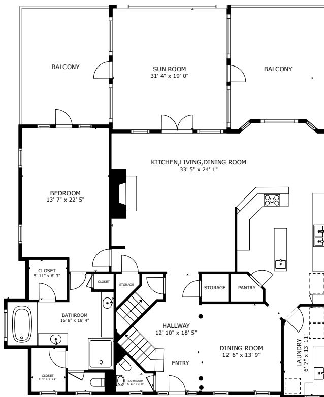
FLOOR 2
