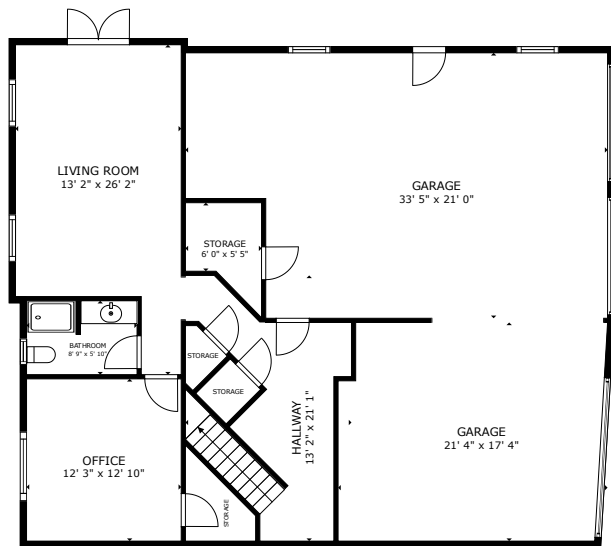
FLOOR 1
