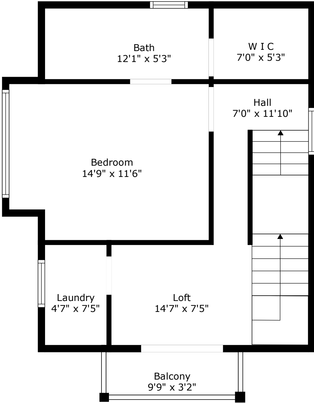
Floor 3
