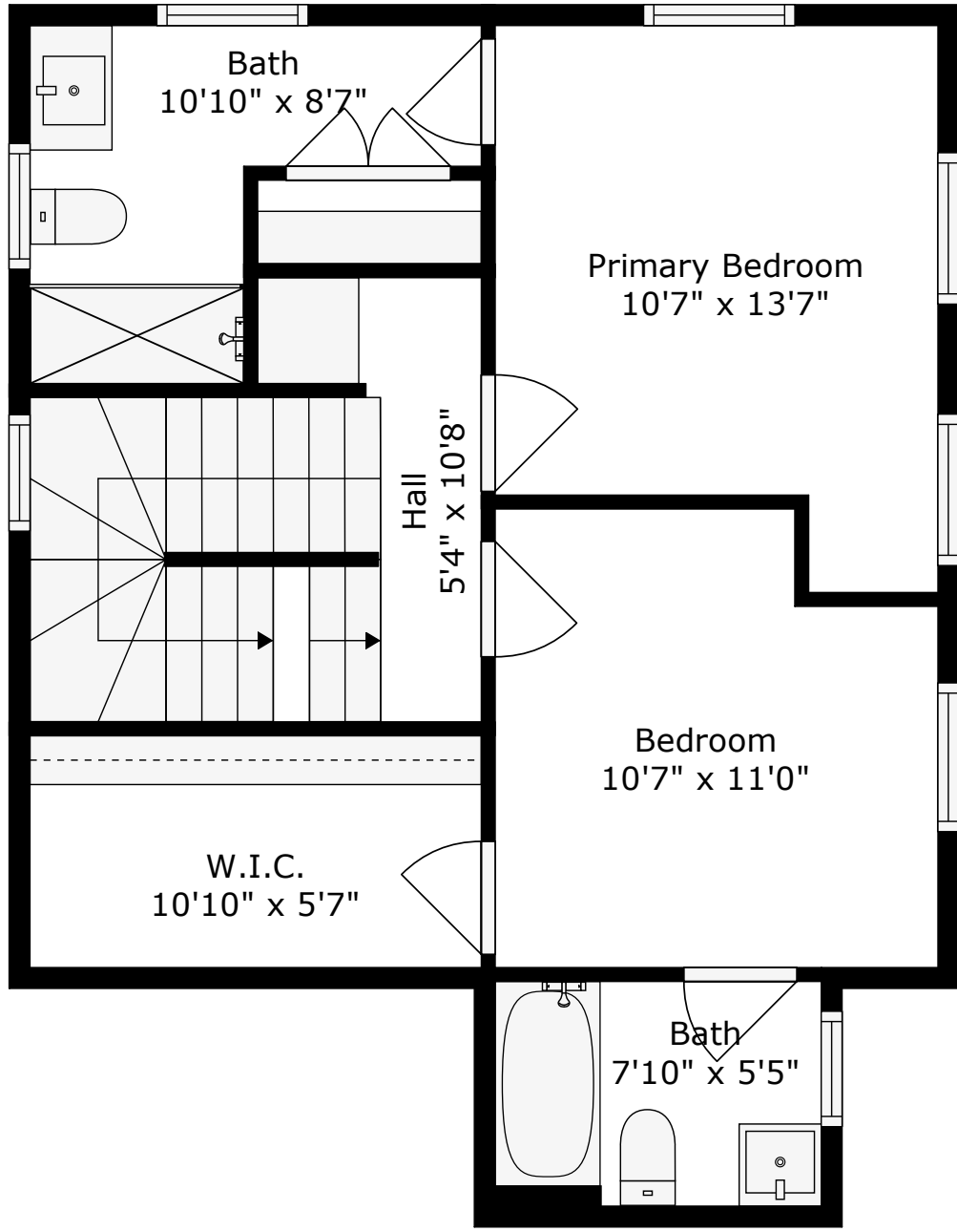
Floor 2
