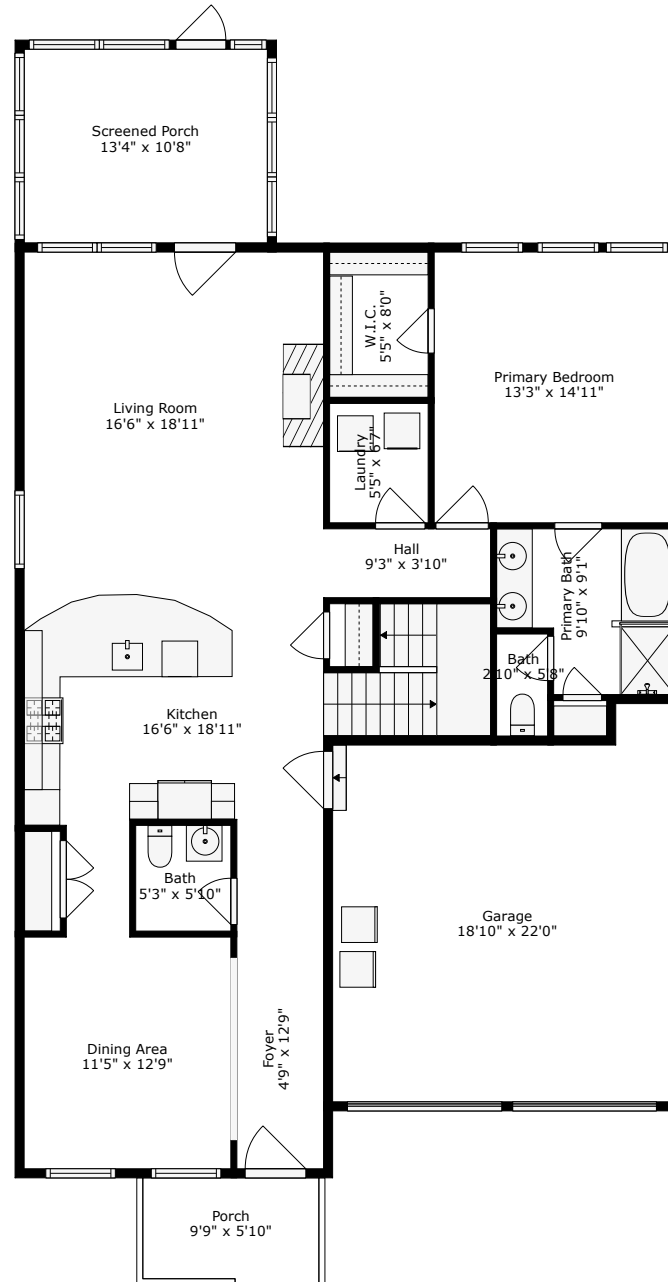
Floor 1
