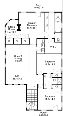
Second Floor
