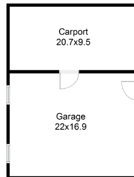
Detached Garage
