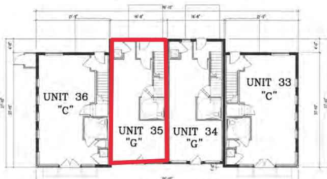
FIRST-FLOOR PLAN
