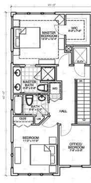
Second Floor 784 sq ft
