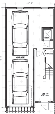
Ground Floor 784 sq ft
